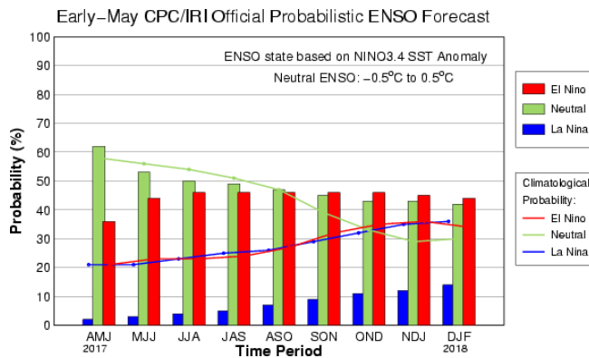
ENSO Probabilities, Valid early May 2017. Source: http://iri.columbia.edu/our-expertise/climate/forecasts/ens0/current/
