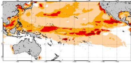
2017 May 2 NOAA Coral Reef Watch 90% Probability Coral Bleaching Thermal Stress for May-Aug 2017
