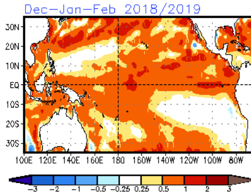
Sea-Surface Temperature Anomalies for Dec-Feb 2018/2019. Source: http://www.cpc.ncep.noaa.gov/
